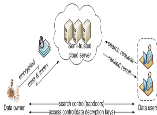
Fig1: architecture
